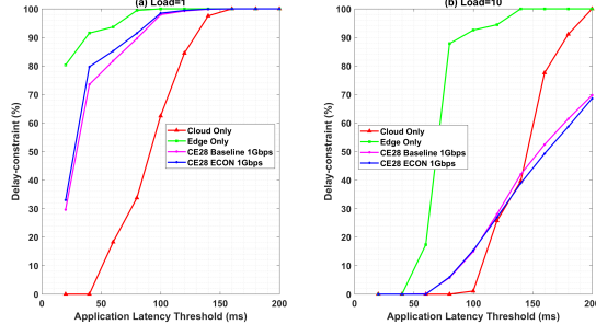
Figure 16. Edge Cloud System Capacity for Different Load and Edge Favored Resources (Inter-edge BW=1 Gbps)
